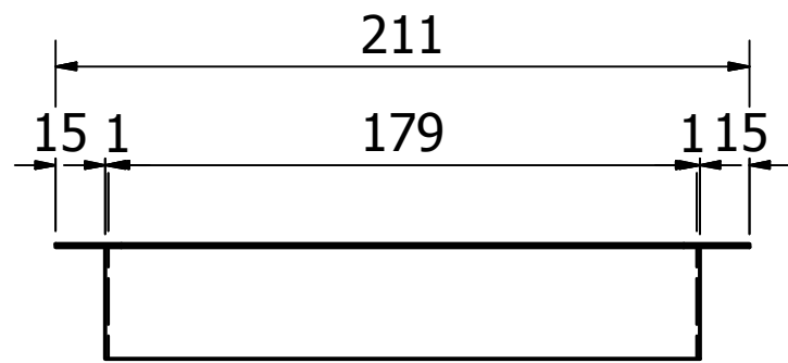
VISTA FRONTAL
