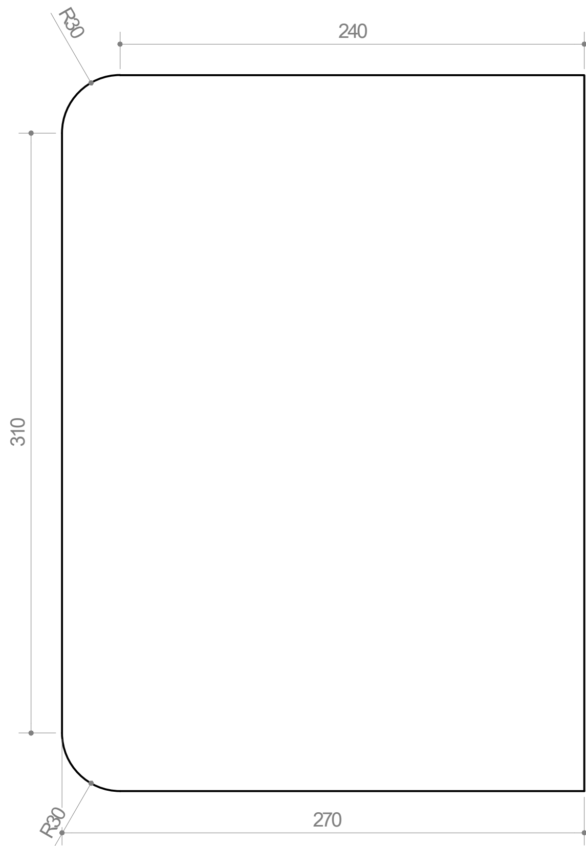
Vista frontal
