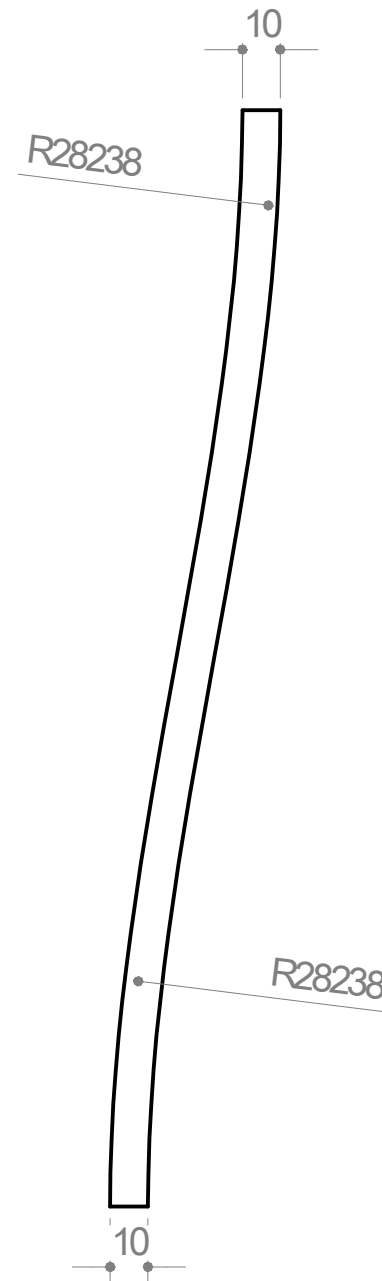
Vista frontal
