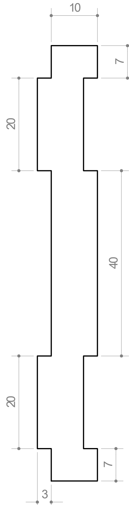
Vista frontal
