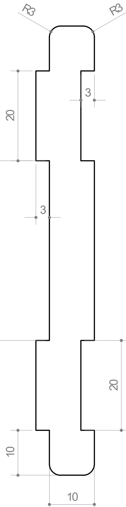
Vista frontal
