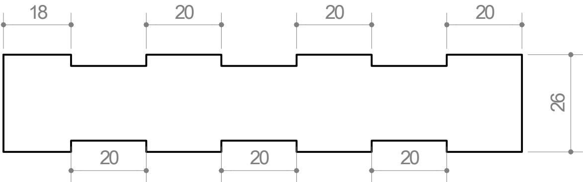
Vista frontal
