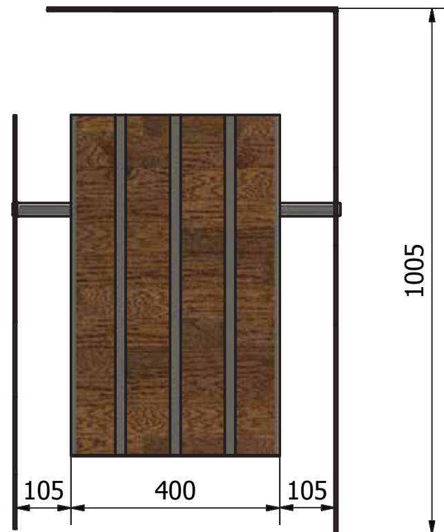
VISTA FRONTAL
