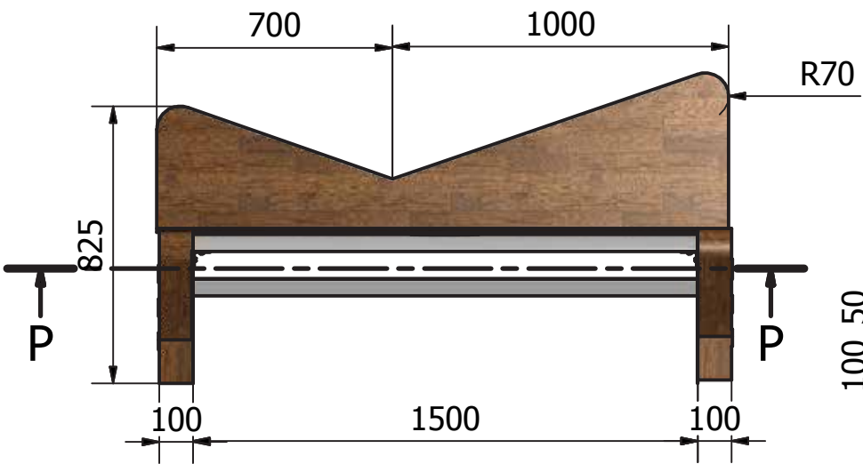
VISTA FRONTAL
