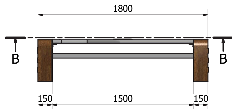
VISTA FRONTAL
