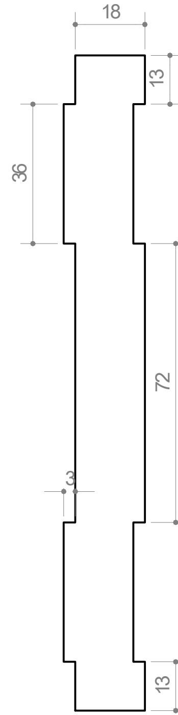
Vista frontal
