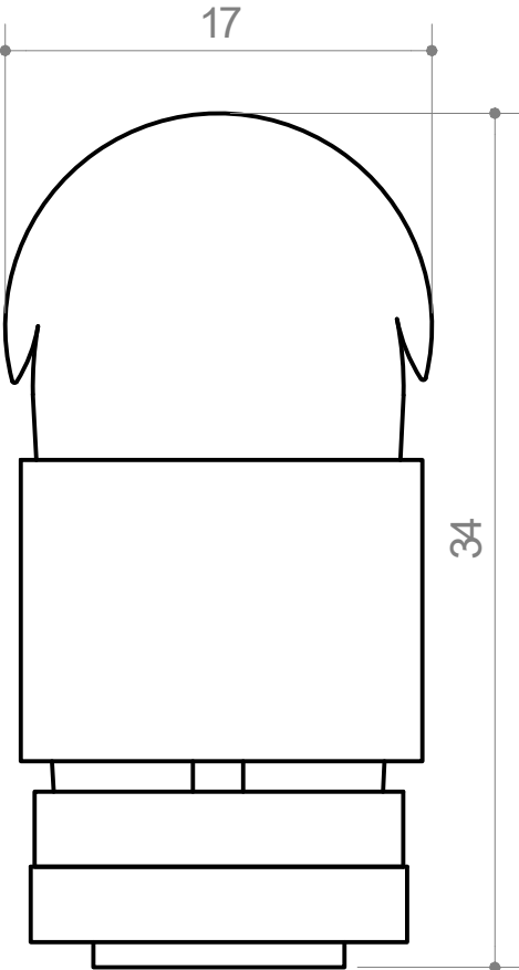
Vista frontal
